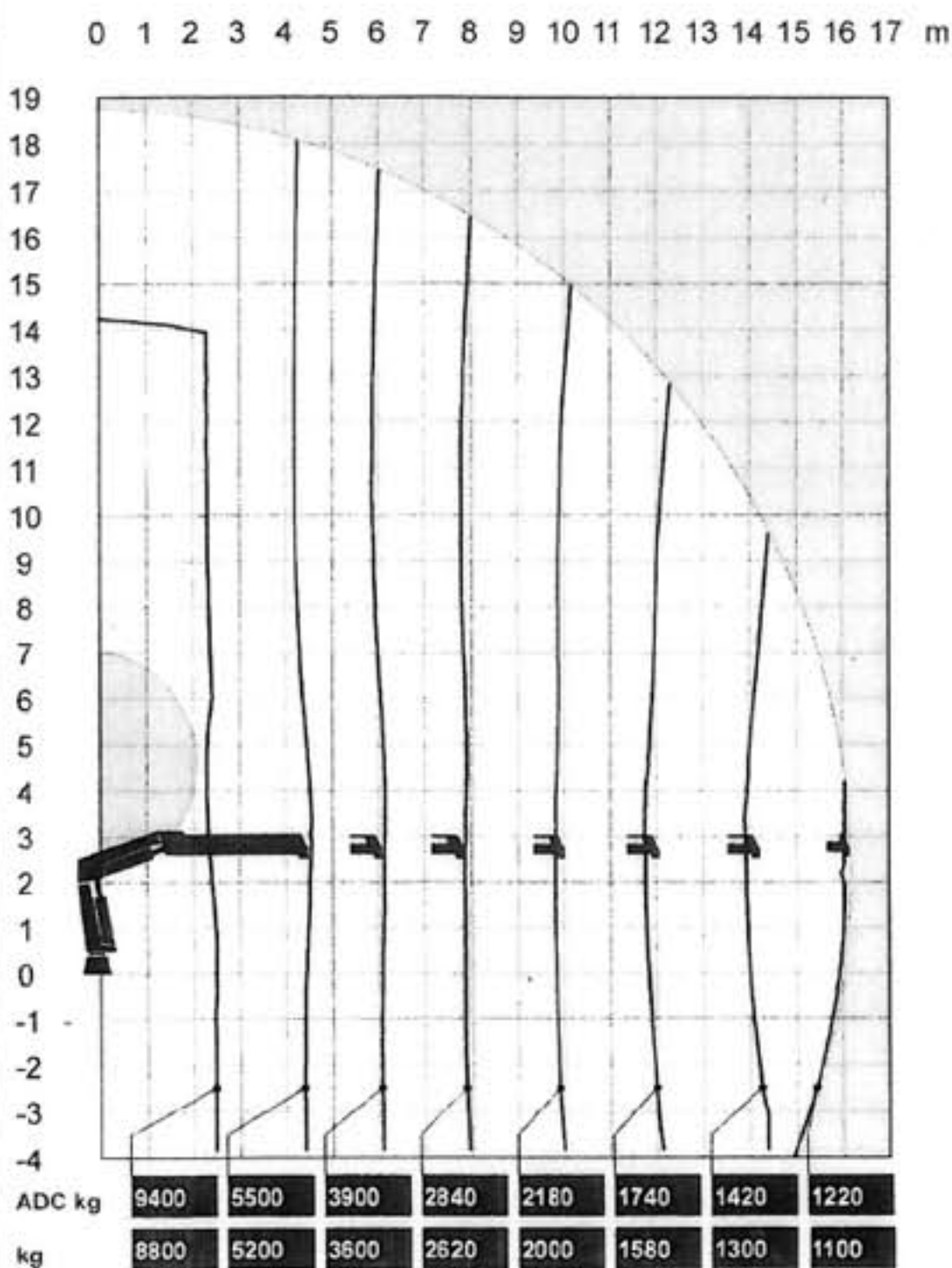
Load diagram
